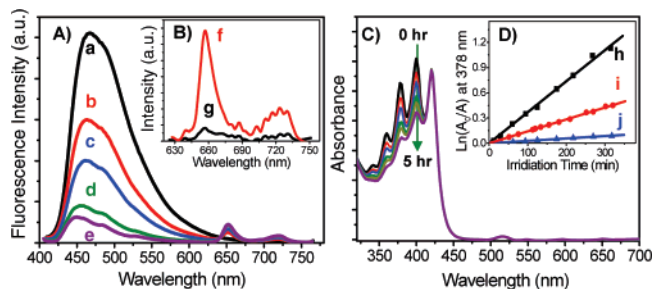
Figure 2. (A) The fluorescence spectra of 1 in P1 with various loading ratio ( 1/P1 in mole: 0, 0.1, 0.2, 0.6, and 1 for curves of a, b, c, d, and e) under the illumination of 380 nm in water. (B) The two-photon-induced emission of 1 in P1 (f) and in P2 (g) with the ratio of 1/1 irradiated at 800 nm. (C) The typical photochemical process of 1/P1/ADPA under the excitation of 800 nm in D_2O . The absorbance of 1 at 420 and 515 nm has no change, indicating the stability of 1 under the experimental condition. (D) The first-order plots for the photooxidation of ADPA in 1/P1/ADPA (curve h), 1/P2/ADPA (curve i), and P1/ADPA (curve j) against irradiation time. A_0 is the absorbance at 378 nm before irradiation. A is the absorbance after irradiation. The ratio of 1 to P1 or P2 in mole is 0.6/1
