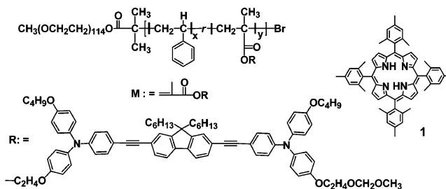
P1 : x = 202 , y = 3 . M_n (GPC) = 18700, M_w/M_n = 1.15 , M_n (NMR) = 29900 P2 : x = 236 , y = 0 . M_n (GPC) = 20400, M_w/M_n = 1.13 , M_n (NMR) = 29500
